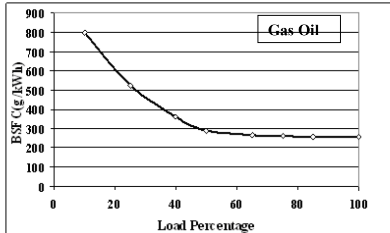
Fig 4: BSFC at constant speed of 1500rpm
