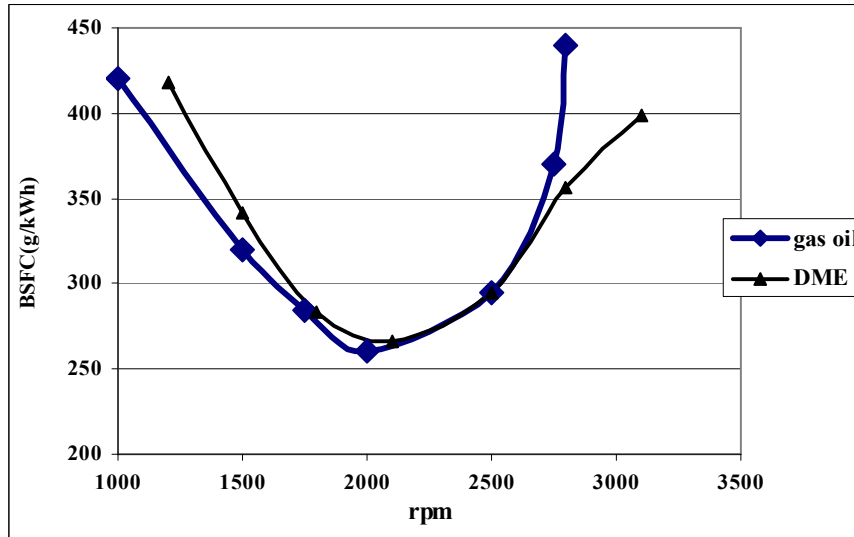
Fig12: Engine Brake Specific fuel consumption (BSFC) with DME and Gas oil at full load.
