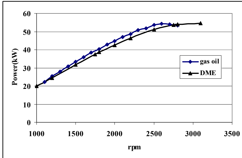
Fig10: Engine power test result with DME and gas oil at full load.
