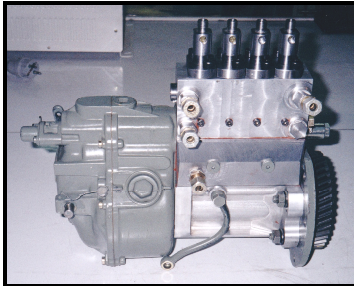
Fig 8: DME fuel pump assembled with engine governor
