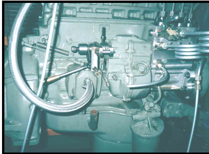
Fig 9: DME fuel injection pump installed on the engine
