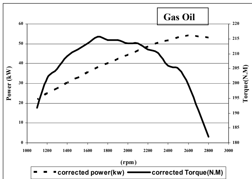
Fig1: Brake power and torque at full load
