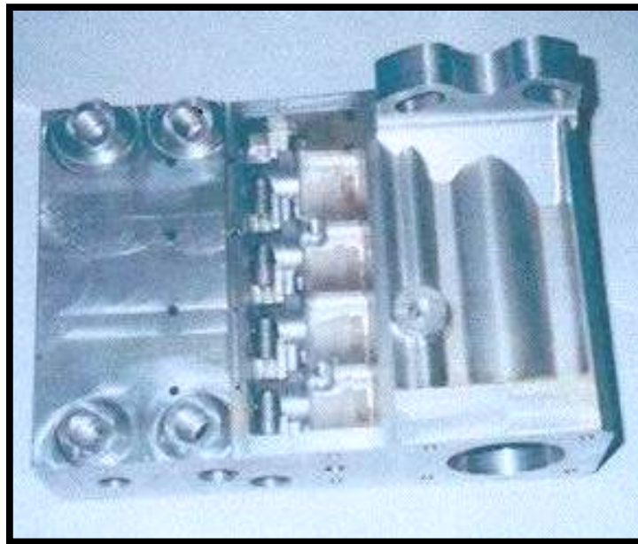
Fig 6: DME fuel pump cylinder block
