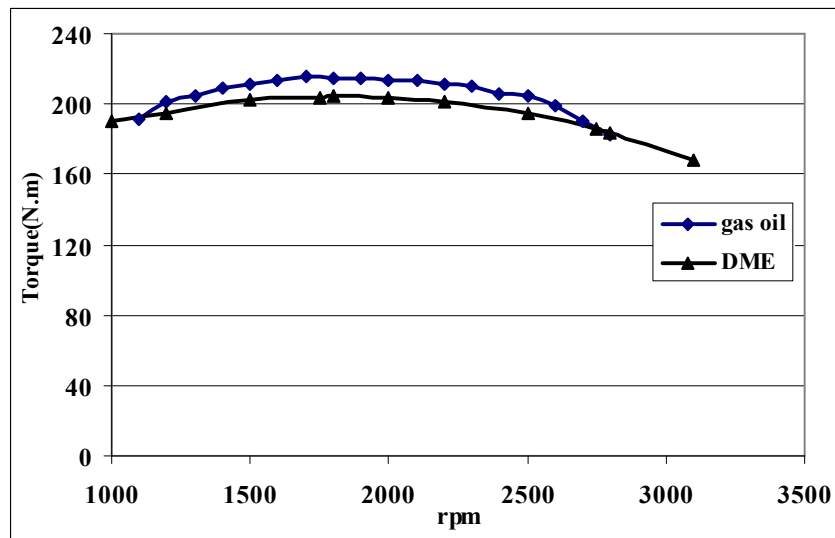
Fig11: Engine torque test result with DME and gas oil at full load.
