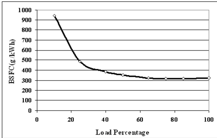
Fig2: BSFC at constant speed of 2500rpm
